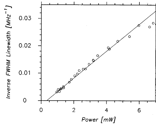
Fig. 4. The inverse of the measured linewidth plotted as a function of the total output from both facets.
